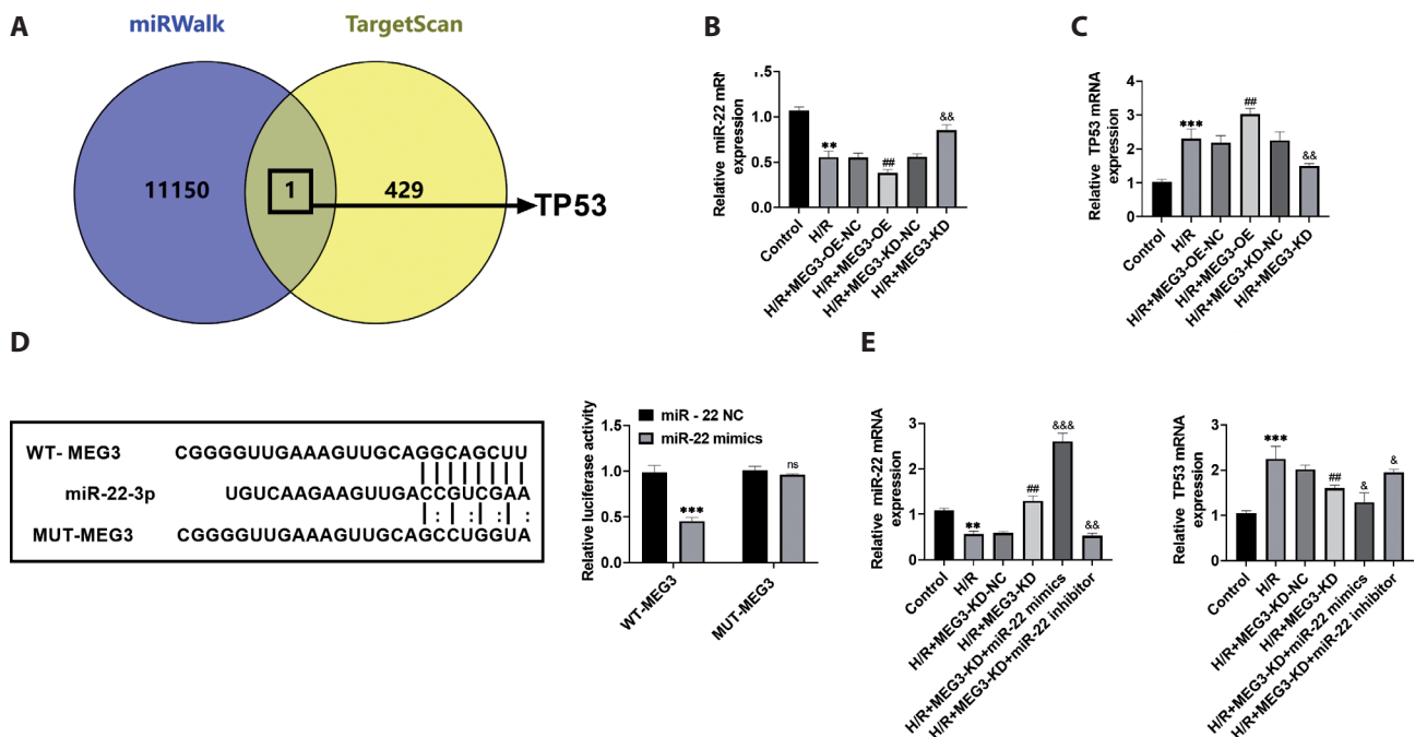
Figure 4. lncRNA MEG3 can mediate miR-22/TP53 signaling. A. Prediction of miR-22-3p target genes by TargetScan and miRWalk databases. H/R treatment caused a decreased miR-22 level ( B ) and raised TP53 level ( C ) in H9C2 cells as measured by qRT-PCR. Overexpression of MEG3 further enhanced the influence of H/R, while knockdown of MEG3 attenuated the impact of H/R. D. Dual luciferase assay confirmed miR-22 as a target of lncRNA MEG3. E. H/R treatment reduced miR-22 levels and increased TP53 expression as measured by qRT-PCR, whereas knockdown of MEG3 resulted in increased miR-22 levels and decreased TP53 levels, and transfection with miR-22 mimics up-regulated miR-22 level and decreased TP53, whereas the opposite was true for transfection with miR-22 inhibitor. n = 5 , **p < 0.01 , ***p < 0.001 vs. Control; \#p < 0.05 , ##p < 0.01 , ###p < 0.001 vs. H/R+MEG3-OE-NC; \&\&p < 0.01 vs. H/R+MEG3-KD-NC.
