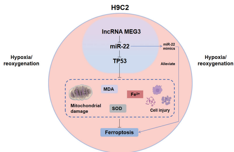
Figure 7. Mechanism of action hypoxia/reoxygenation-induced ferroptosis. IncRNA MEG3 expression was upregulated in H9C2 cells caused by H/R, and it promoted H/R-caused cell injury and ferroptosis by regulating miR-22/TP53 signaling.
