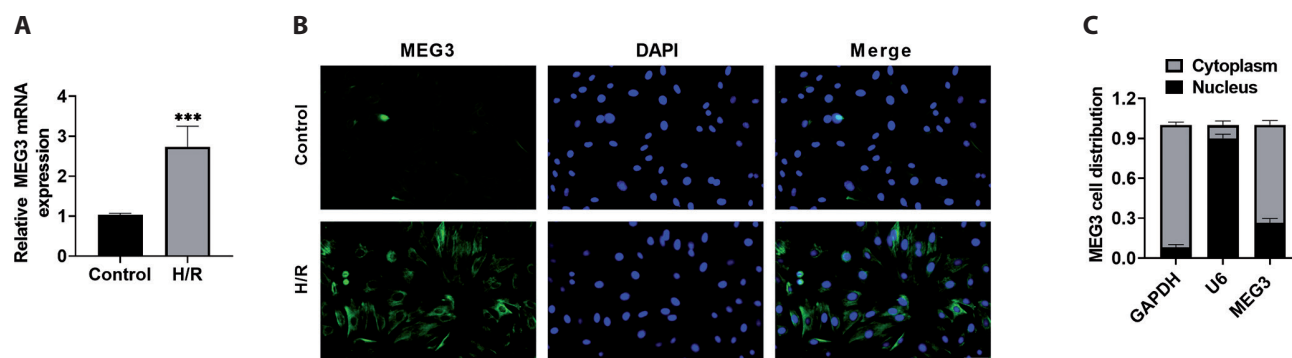
Figure 1. lncRNA MEG3 is upregulated in H/R-induced H9C2 cells. A. MEG3 RNA expression in H9C2 cells after H/R treatment was assessed through qRT-PCR. B. RNA FISH confirmed that RNA expression of MEG3 was elevated after H/R treatment and located in the cytoplasm (40 \times , 50 \mu m). C. MEG3 RNA expression in the nucleus and cytoplasm was detected via qRT-PCR, which suggested that MEG3 was expressed mainly in the cytoplasm. n = 5 , *** p < 0.001 vs. Control.
