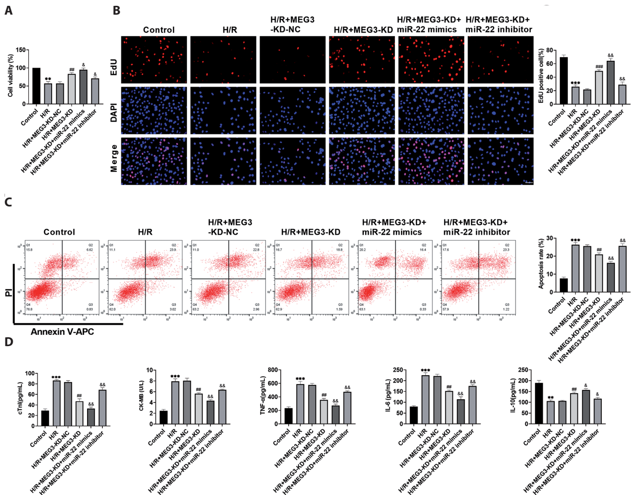
Figure 5. IncRNA MEG3 mediates miR-22/TP53 signaling to promote H9C2 cell injury induced by H/R. A. CCK-8 assay showed that knockdown of MEG3 increased cell viability, which was further raised by transfection of miR-22 mimics, while the opposite was true for transfection of miR-22 inhibitor. B. EdU staining measured knockdown of MEG3 raised the rate of EdU-positive cells, which was further increased by transfection of miR-22 mimics, while miR-22 inhibitor decreased EdU-positive cells (40×, 50 μm). C. Knockdown of MEG3 resulted in decreased apoptosis as measured through flow cytometry, which was further decreased by transfection of miR-22 mimics, while miR-22 inhibitor raised the apoptosis rate. D. Knockdown of MEG3 decreased cTnI, CK-MB, IL-6 and TNF-α levels and raised IL-10 level as assessed by ELISA kits, and transfection of miR-22 mimics further raised the impact of knockdown MEG3, while miR-22 inhibitor did the opposite. n = 5 , *** p < 0.001 vs Control; ## p < 0.01 , ### p < 0.001 vs H/R+MEG3-KD-NC; & p < 0.05 , && p < 0.01 vs H/R+MEG3-KD.
